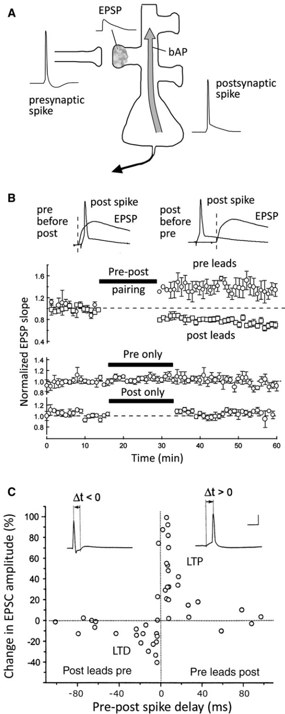
Figure 1. Spike-Timing-Dependent Plasticity
